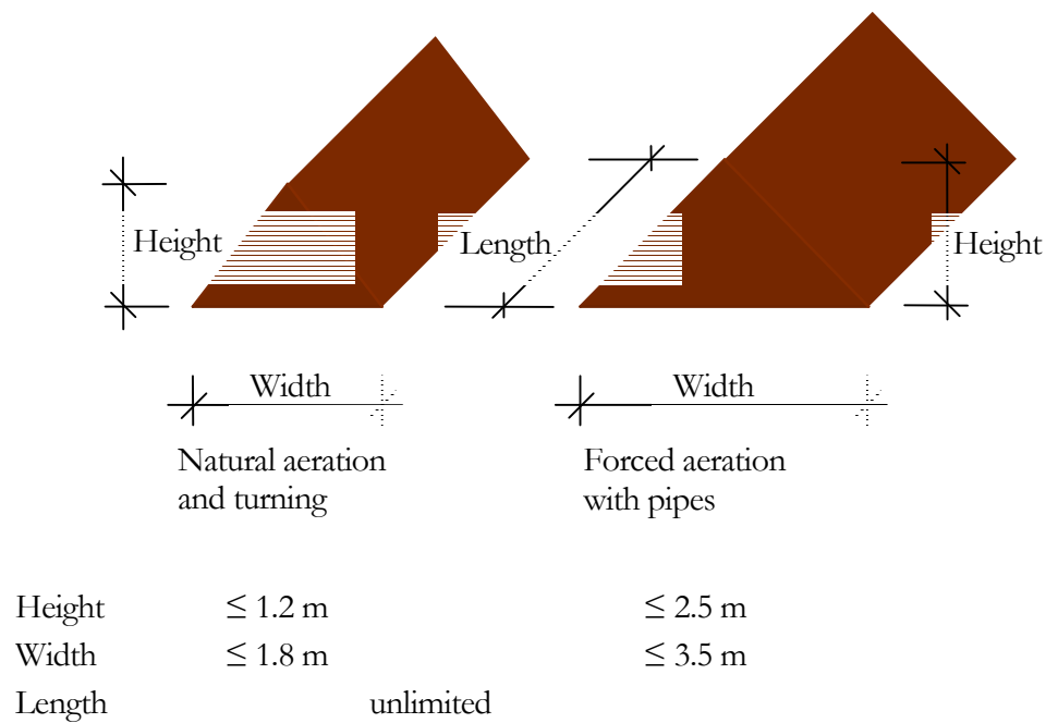
Figure III-1 Windrow dimensions depending on the aeration system
